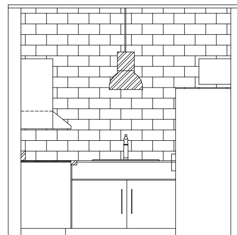
KITCHEN ELEVATION SCALE: \frac{1}{4}" = 1'-0"
