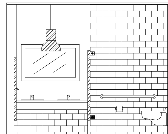
GIRLS' BATHROOM ELEVATION SCALE: \frac{1}{4}" = 1'-0"
